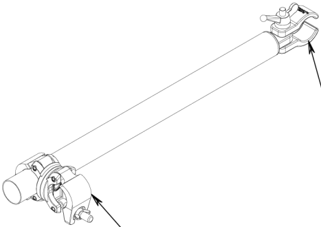
Swivel coupler to tie to unit
